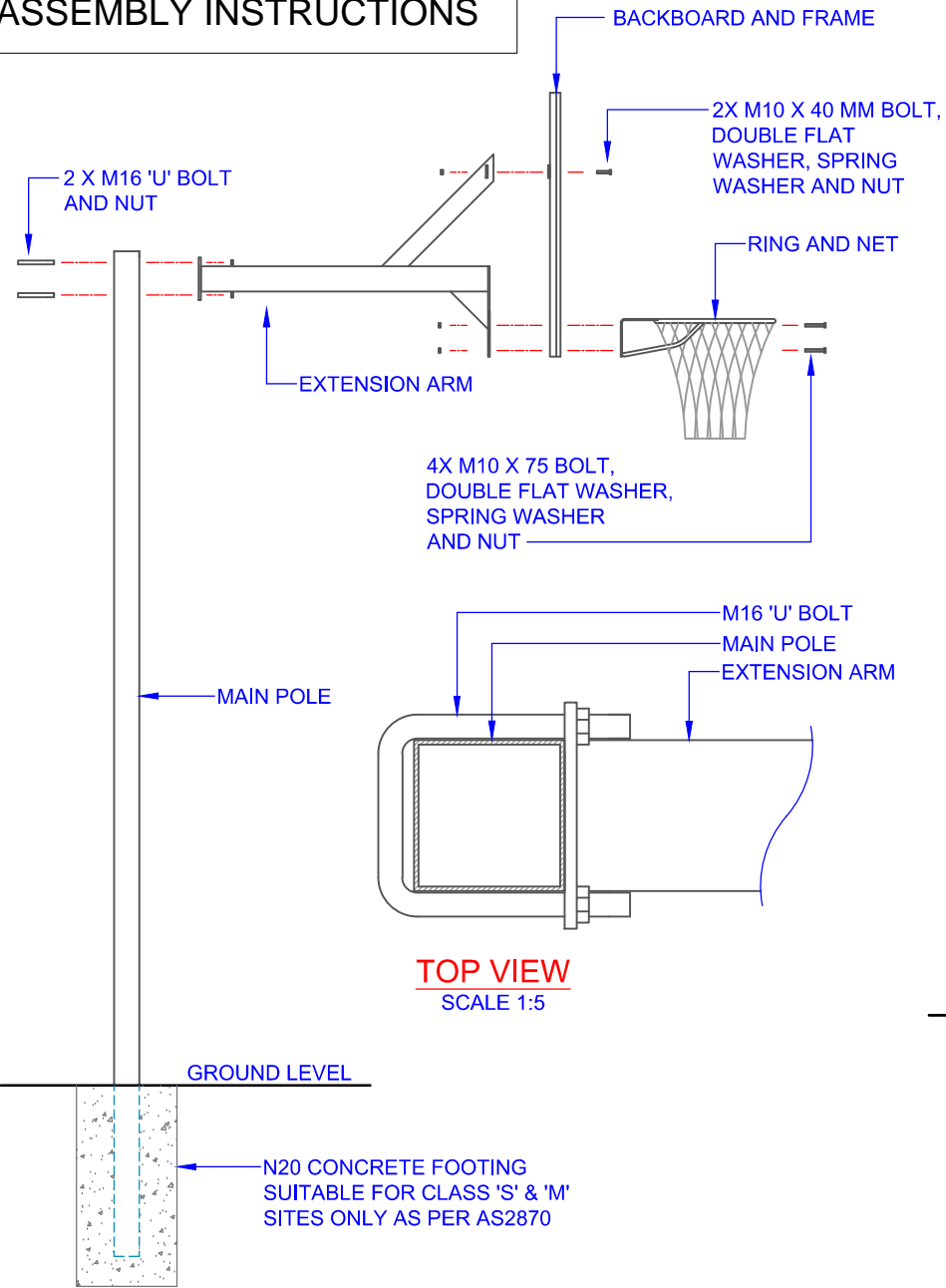
FORCE 10 BASKETBALL TOWER SCALE 1:30
