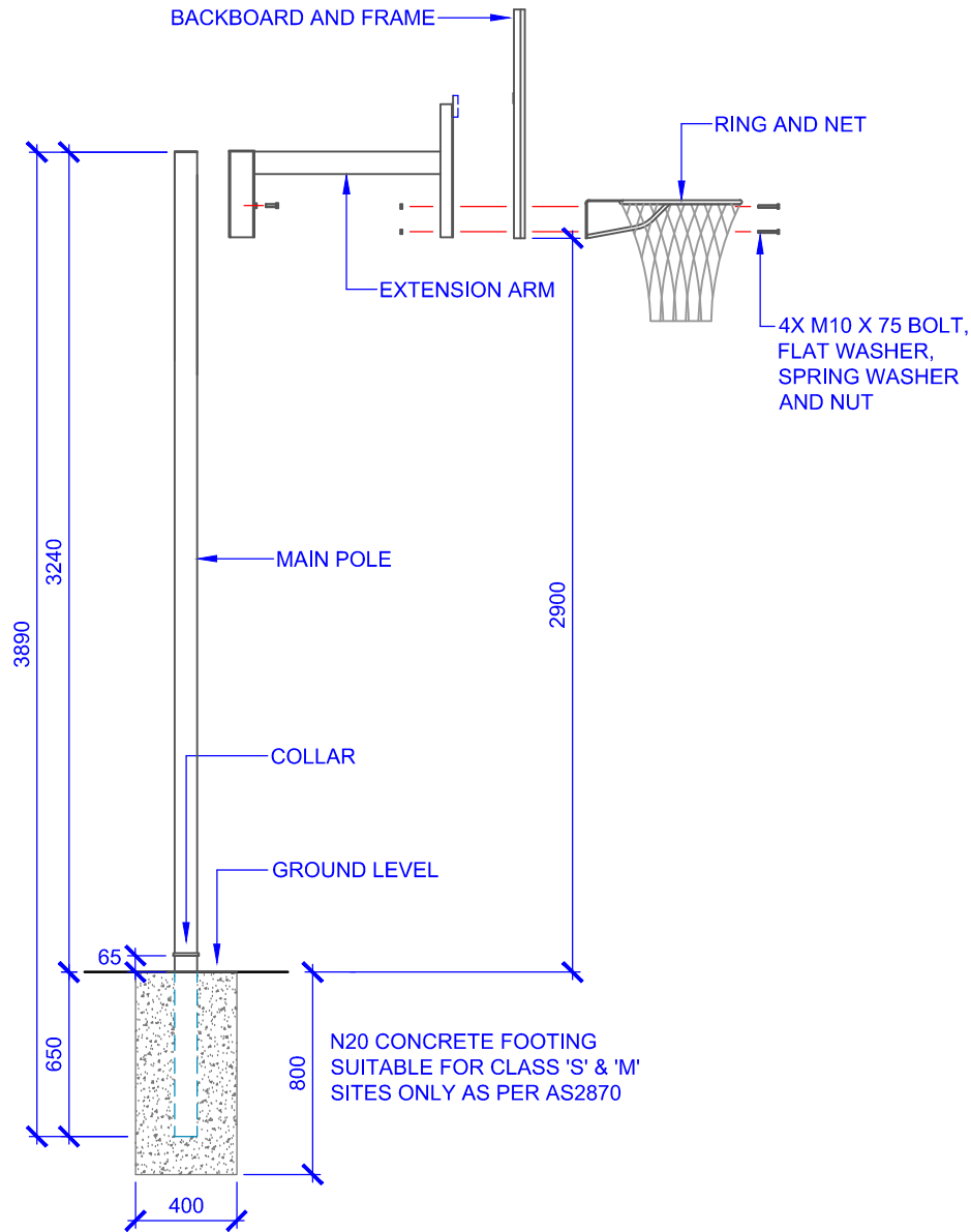
LEGEND BASKETBALL TOWER WITHOUT GROUND SLEEVE SCALE 1:30
