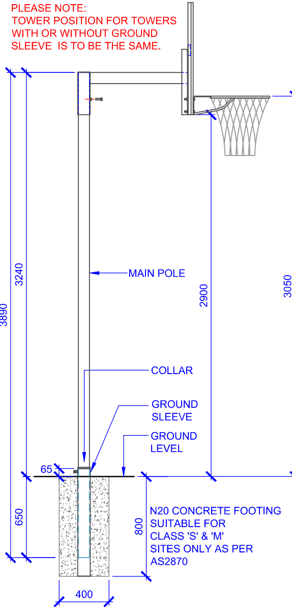
LEGEND BASKETBALL TOWER WITH GROUND SLEEVE SCALE 1:30
