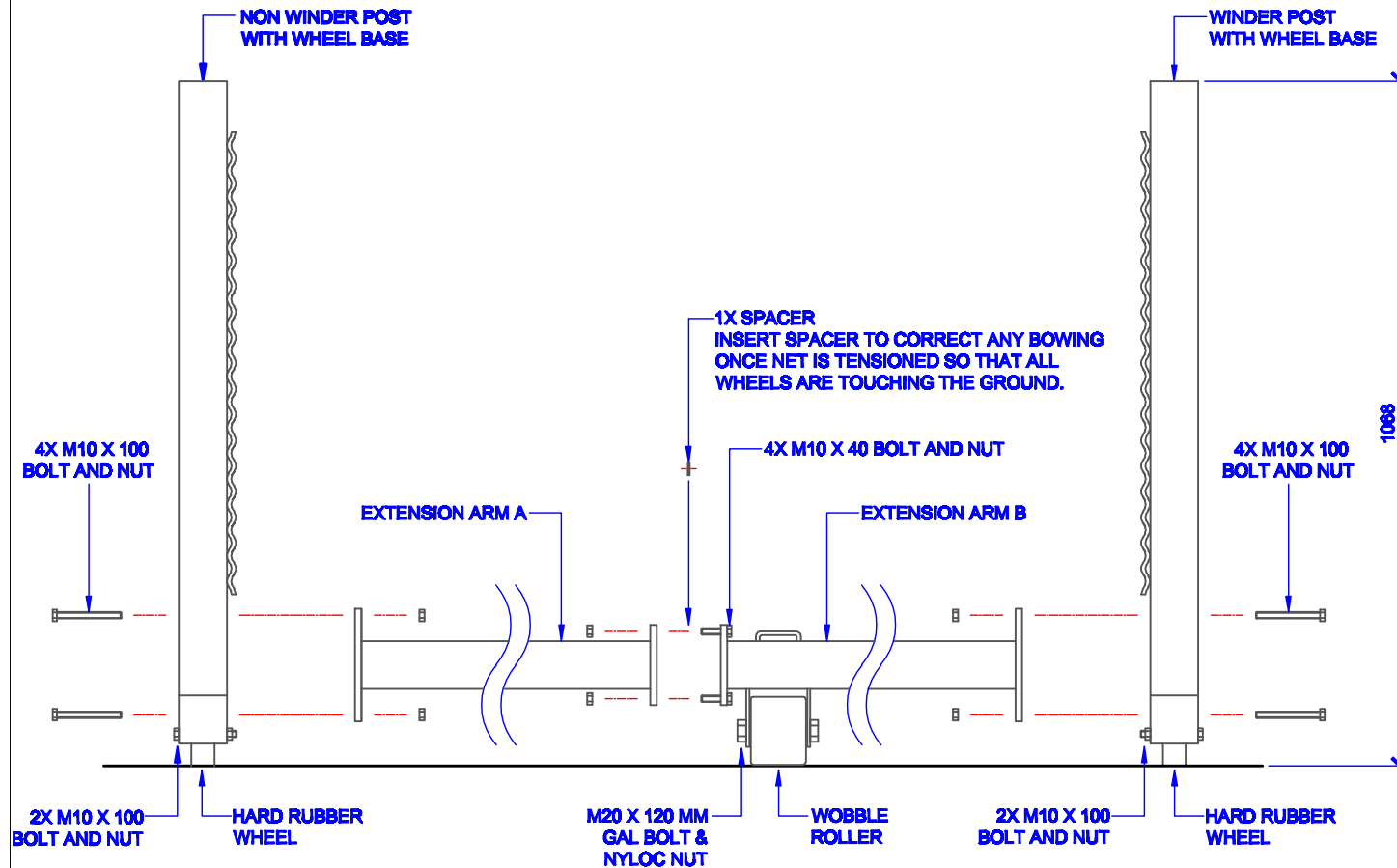
TPF75 FREESTANDING NET POSTS SCALE 1:10
